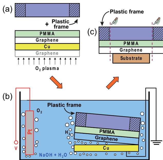
FIG. 1. Schematic illustration of the frame assisted \text{H}_2 bubbling transfer. (a) Deposition of the PET frame on top of the sample and etching of the graphene at the unprotected side of Cu with \text{O}_2 plasma. (b) \text{H}_2 bubbling separation of the frame/PMMA/graphene from the Cu foil induced by \text{H}_2\text{O} electrolysis. (c) Frame removal after transfer.
